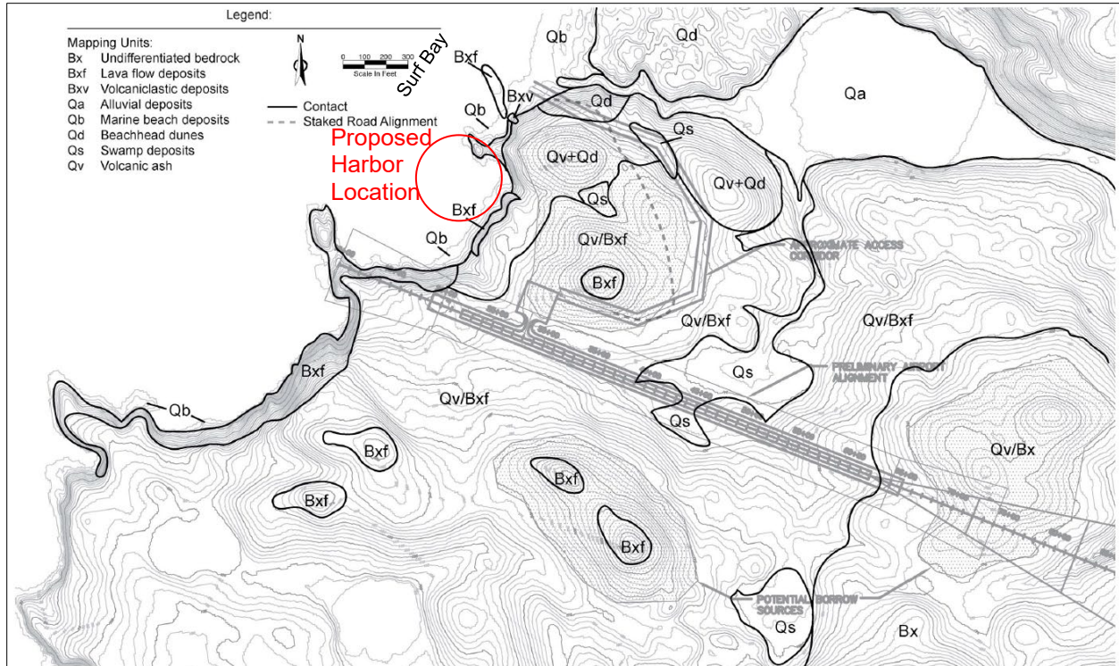
Figure 4-1. Geologic Map of Akutan and Akun Islands (DMA, 2005)
