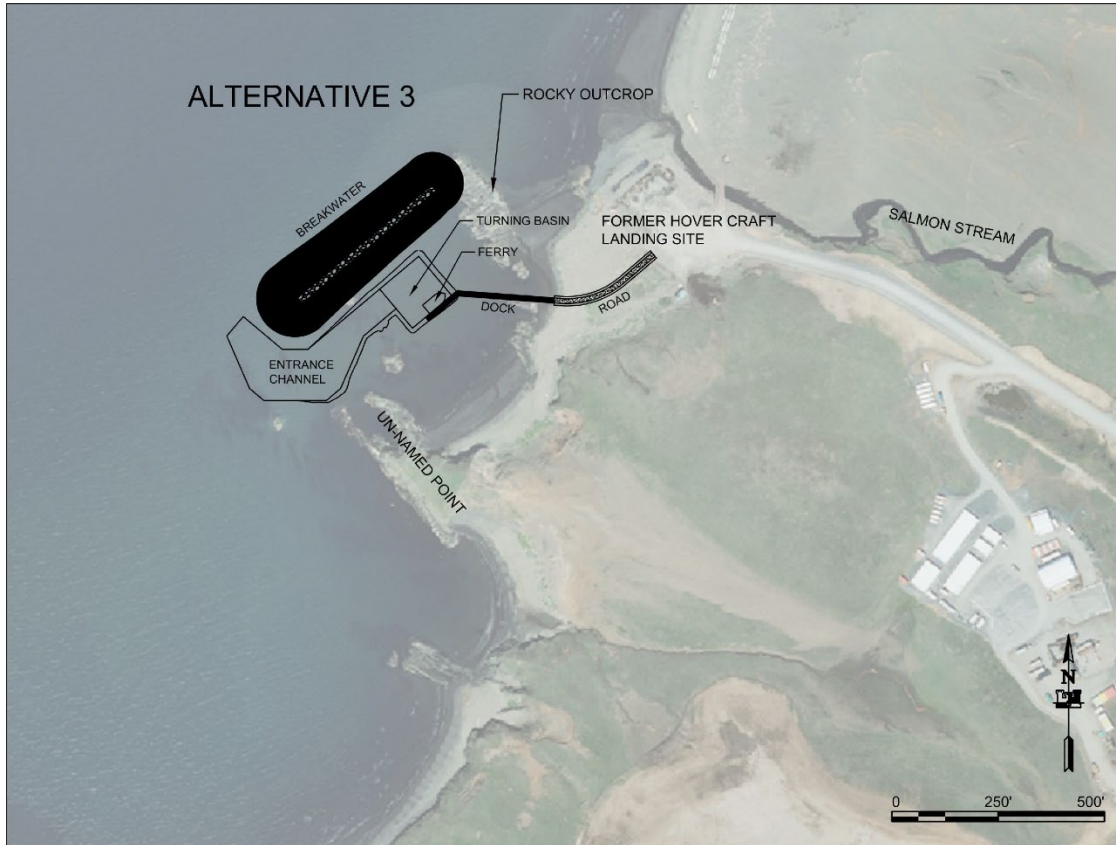
Figure 6-3. Alternative 3: Harbor Located South of Unnamed point (with blasting)
