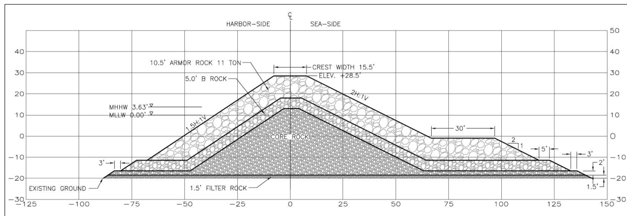
Figure 5-1. Preliminary Breakwater Cross-Section
