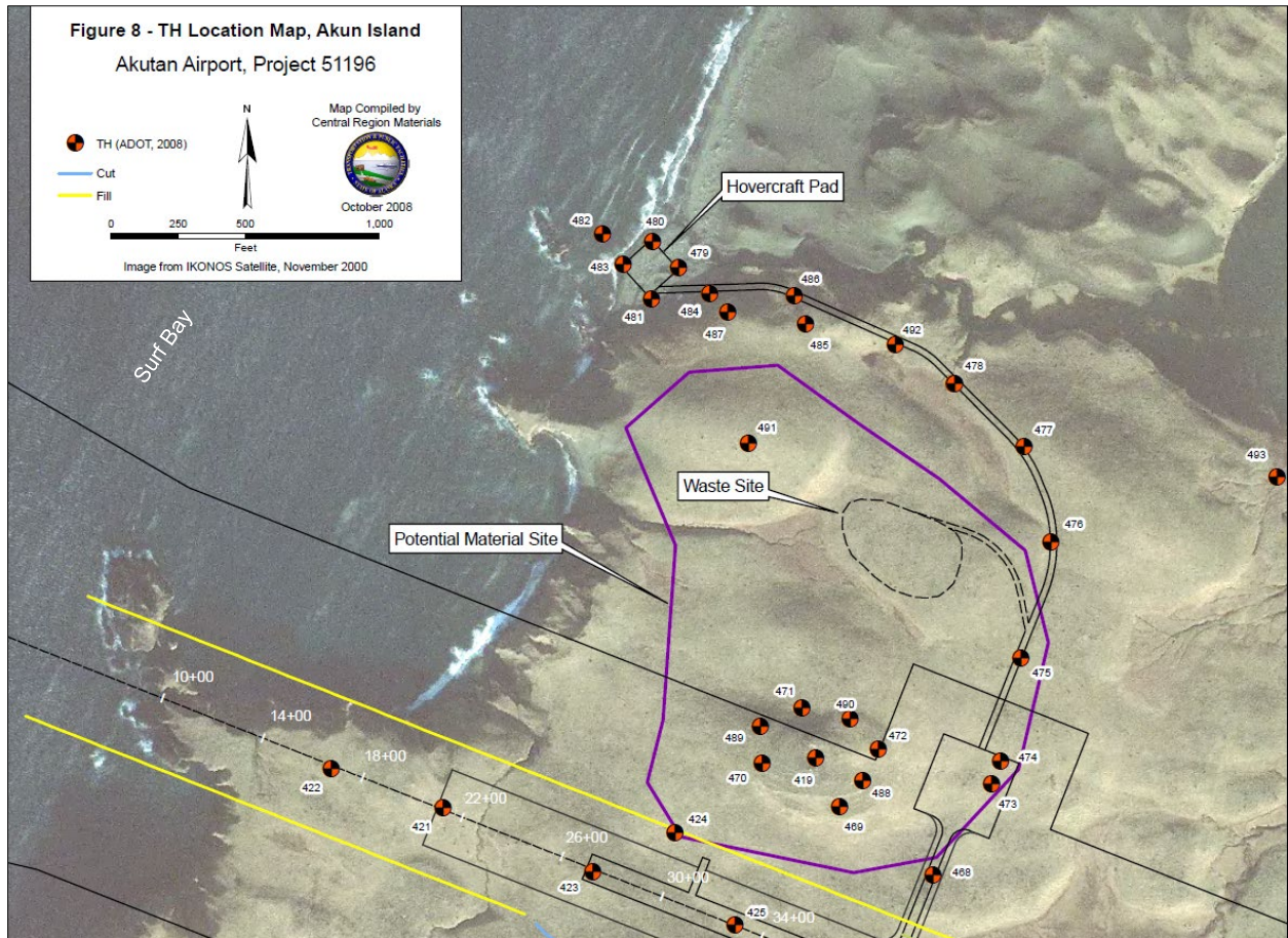
Figure 3-1. Historical Test Boring Locations (ADOT, 2008)
