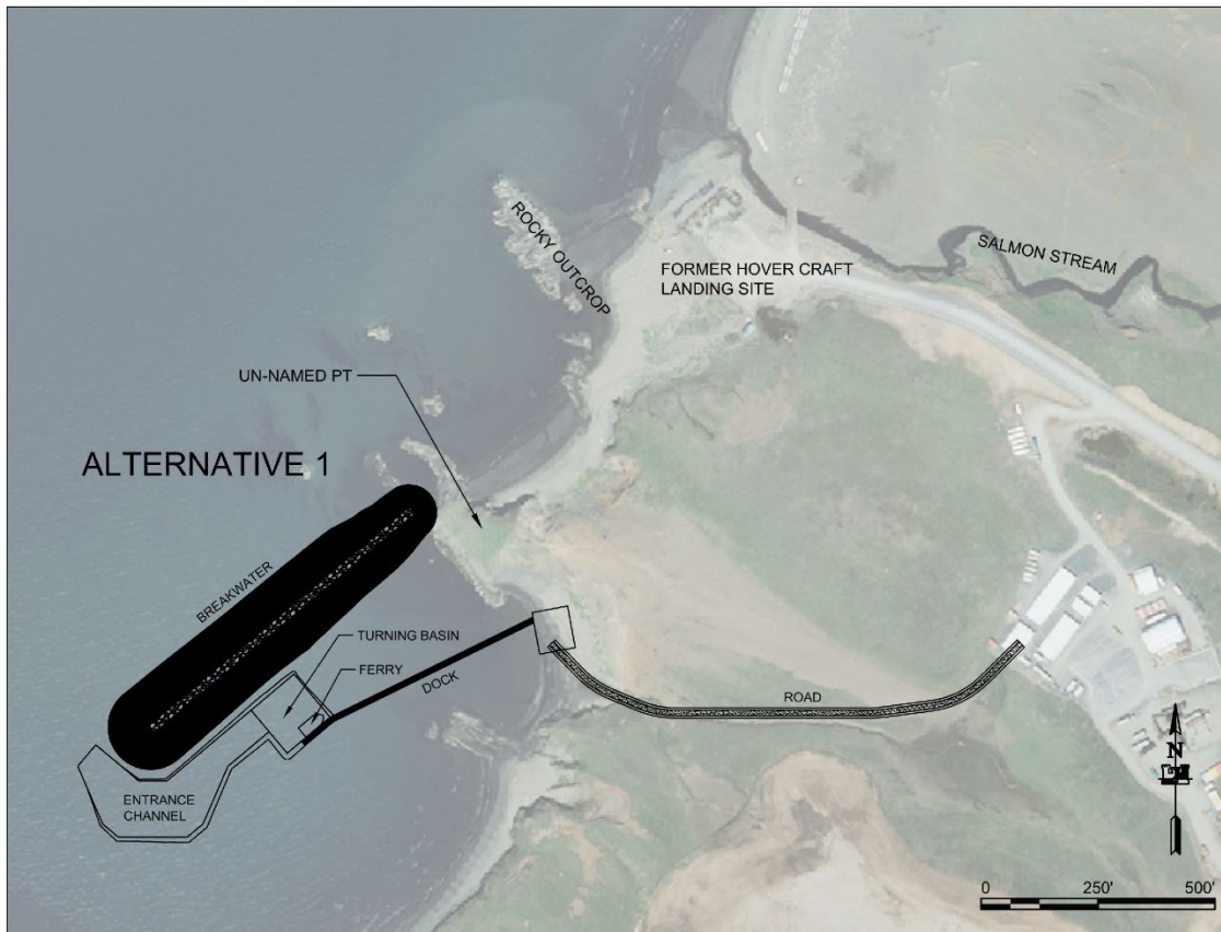
Figure 6-1. Alternative 1: Harbor Southwest of Unnamed Point (without blasting)
