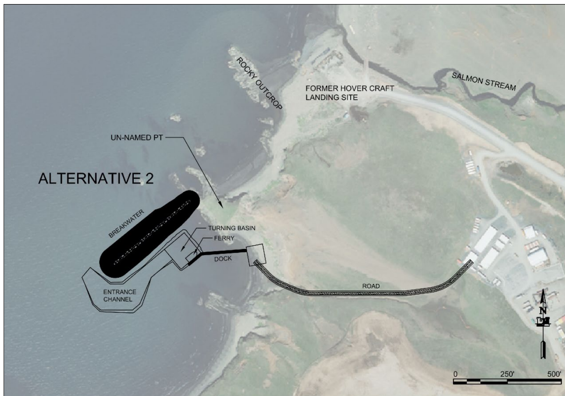
Figure 6-2. Alternative 2: Harbor South of Unnamed Point (with blasting)
