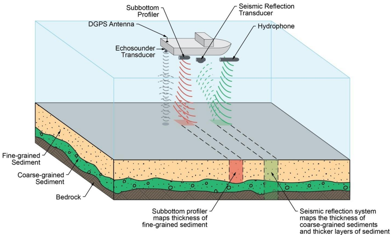
Image 1: Example Survey Instrumentation Schematic. Side Scan Sonar towfish is not shown.
