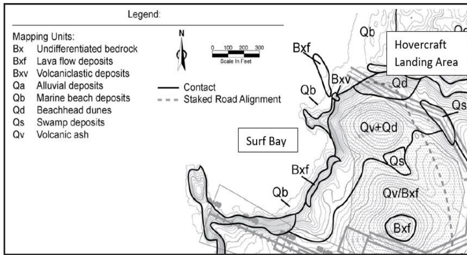
Image 3: Surficial geology at Surf Bay (excerpted from DMA 2005, Plate 1)
