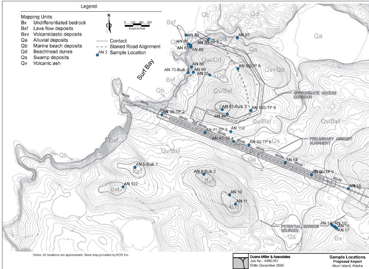
Figure 3-2. Historical Test Boring Locations (DMA, 2005)
